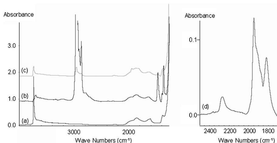
Figure 1. Monitoring the formation of tungsten hydride supported on SiO_2-Al_2O_{3-(500)} ( 3 ) by IR spectroscopy: a) Silica-alumina dehydroxylated at 500^\circ\text{C} . b) [(\equiv SiO)W(\equiv C-t-Bu)(CH_2-t-Bu)_2]_{SA} . c) After treatment under H_2 at 150^\circ\text{C} for 12 h. d) Subtraction of a) from c), zoom of the 2500\text{--}1700\text{ cm}^{-1} region.
