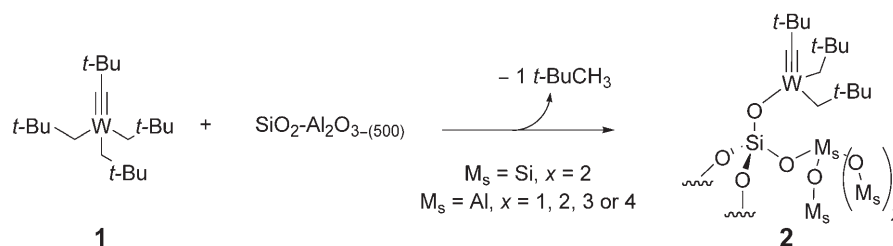
Scheme 1. Grafting of [W(\equiv C-t-Bu)(CH_2-t-Bu)_3] ( 1 ) onto SiO_2-Al_2O_{3-(500)} .
